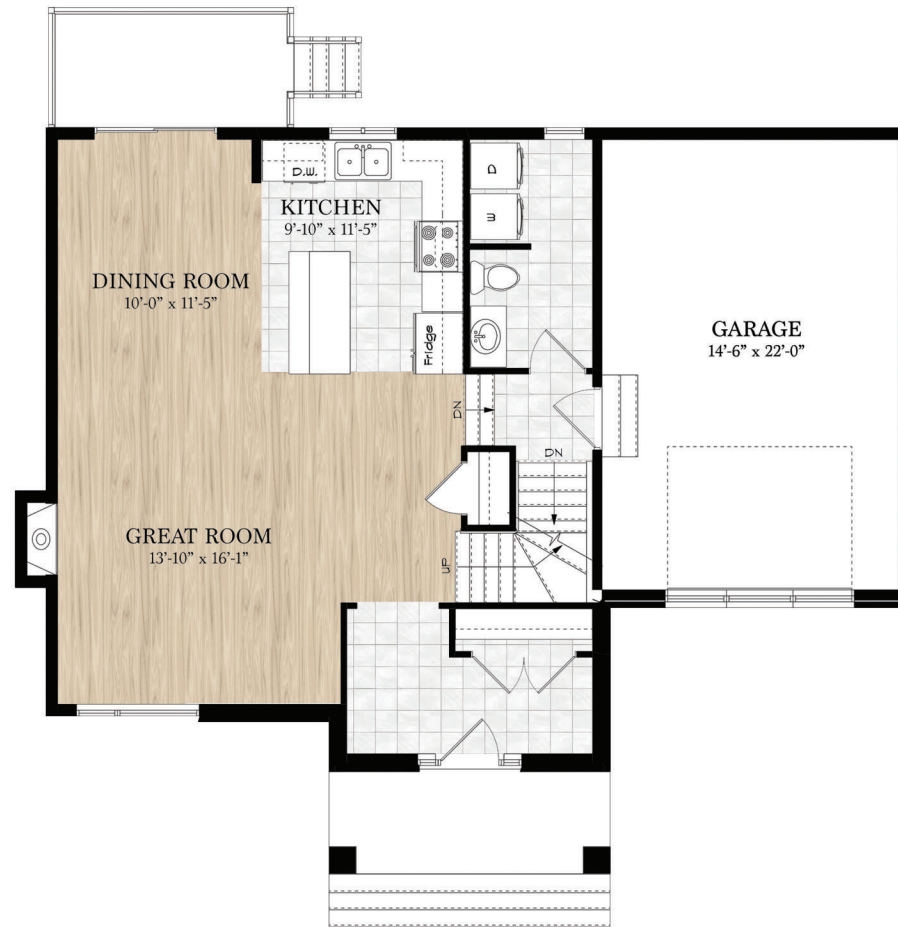
Main Floor Plan Living Area: 1604 sq. ft.
