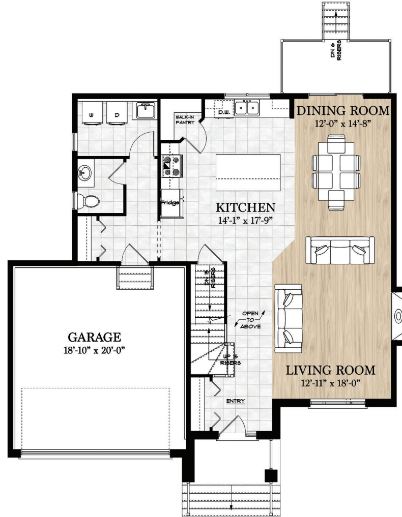
Main Floor Plan Living Area: 2079 sq. ft.
