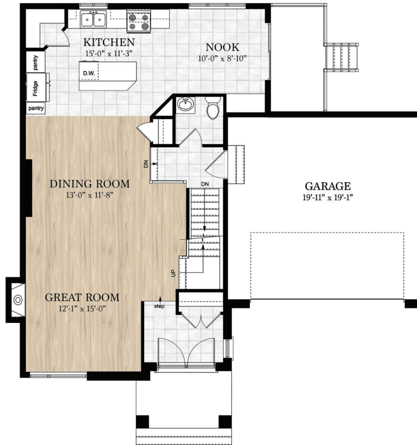
Main Floor Plan Living Area: 2011 sq. ft.
