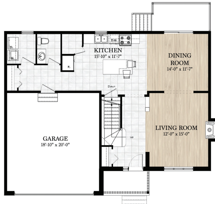
Main Floor Plan 1714 sq. ft.
