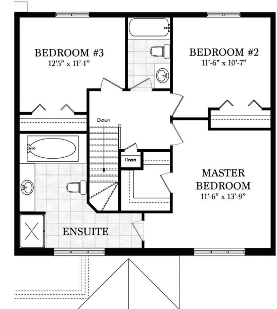
Second Floor Plan - Optional Ensuite
