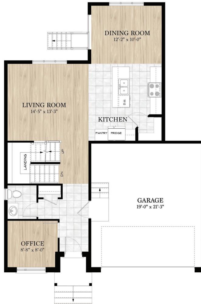
Main Floor Plan Living Area: 1699 sq. ft.
