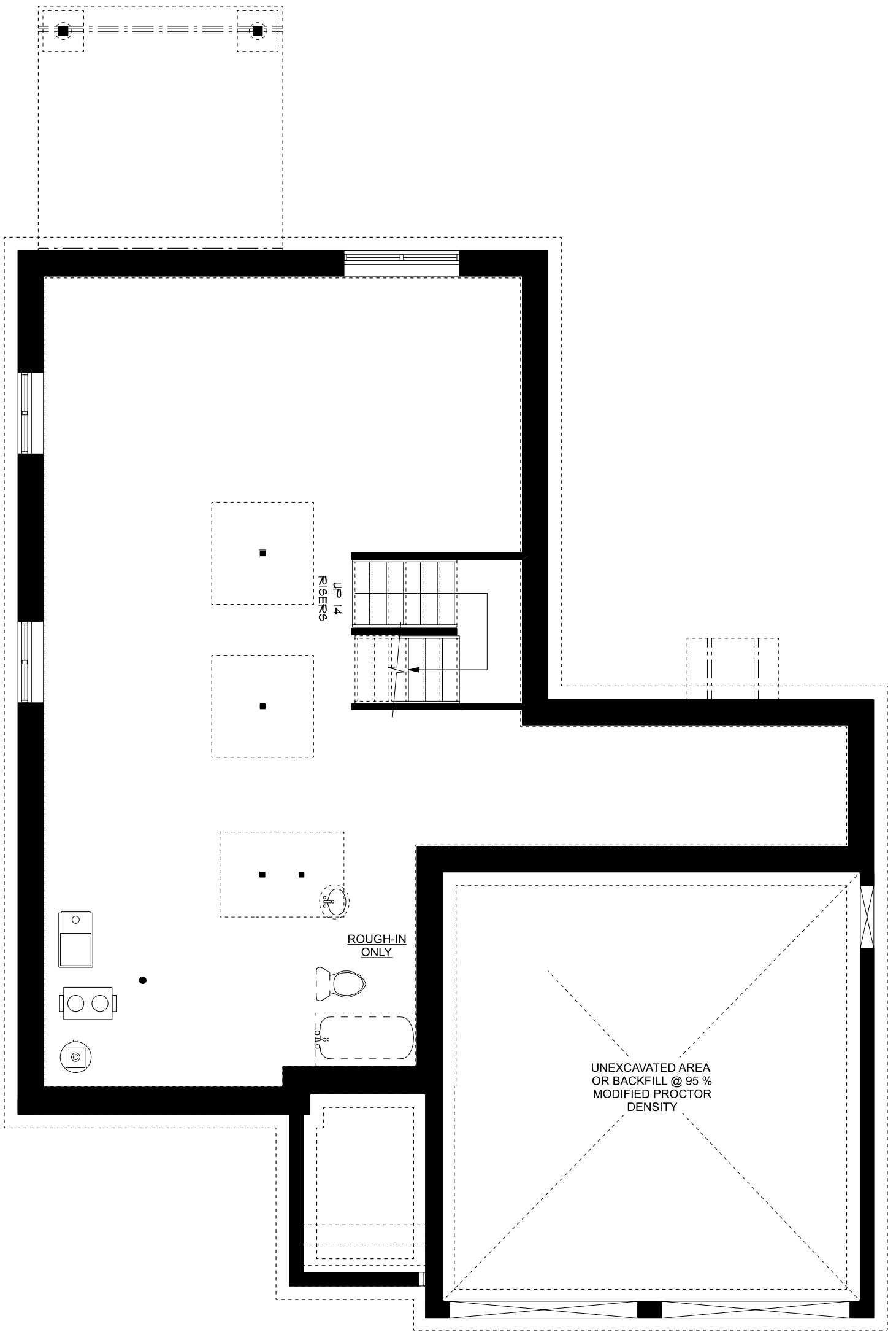
FOUNDATION PLAN
