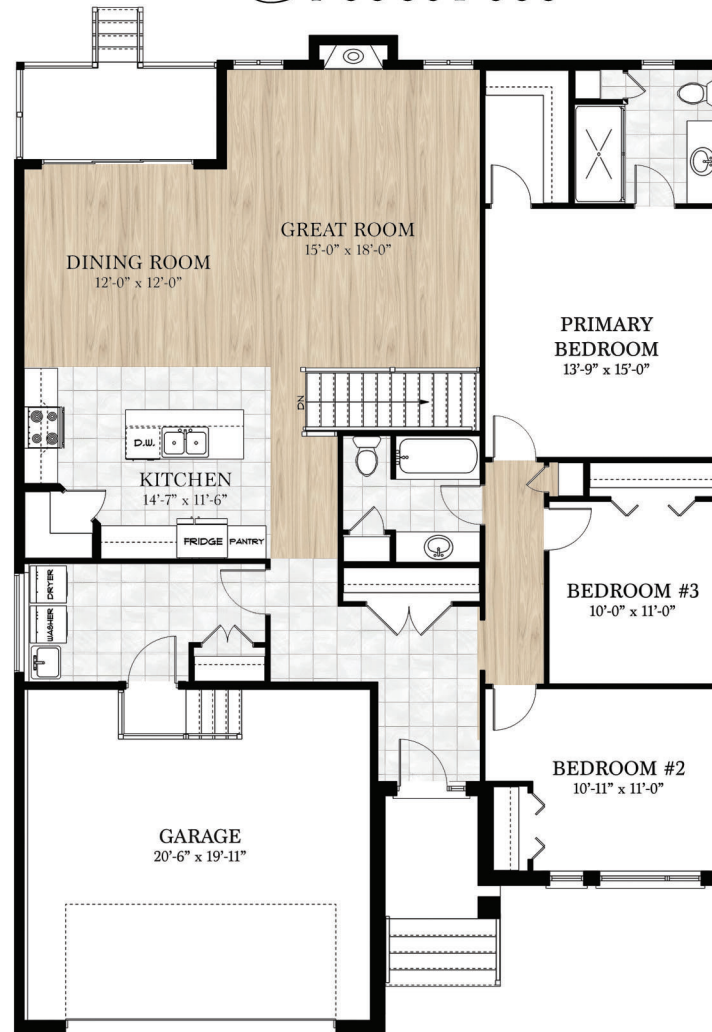
Main Floor Plan Living Area: 1720 sq. ft.
