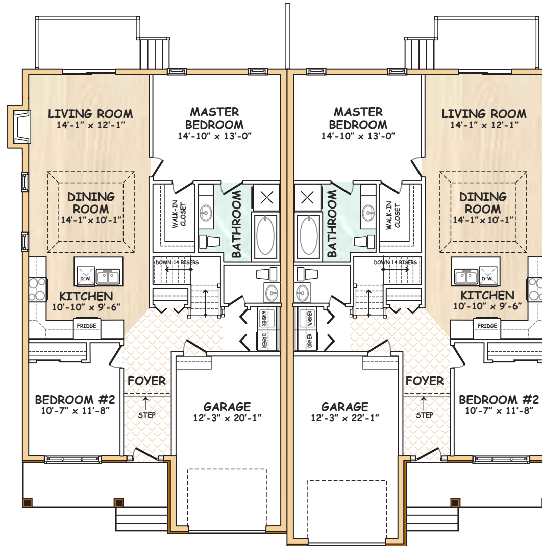
MAIN FLOOR PLAN - EACH UNIT 1258 SQ. FT.
