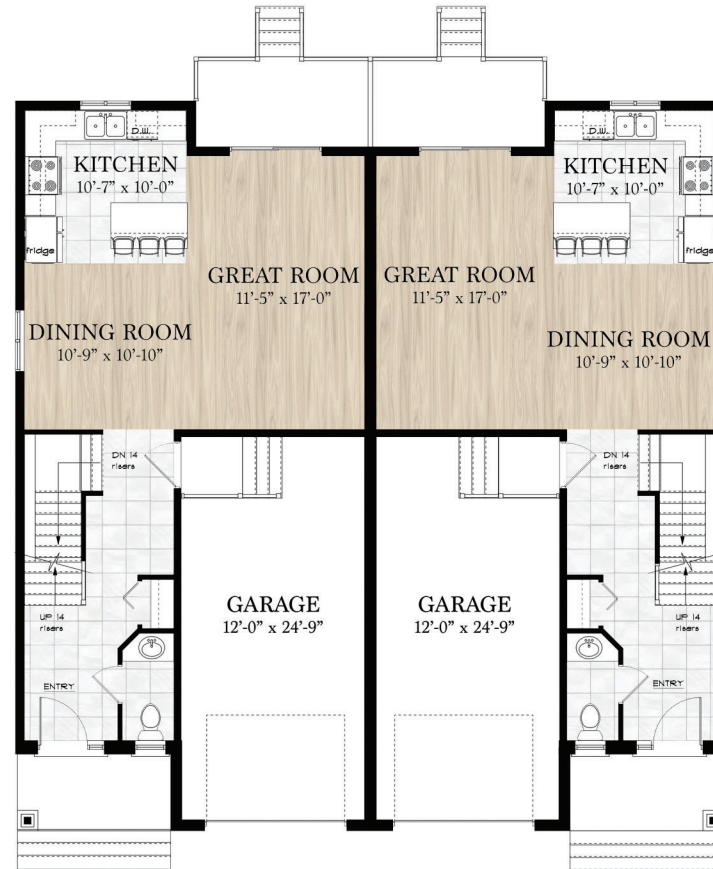
Main Floor Plan Option A: 1642 sq. ft. Option B: 1628 sq. ft.
