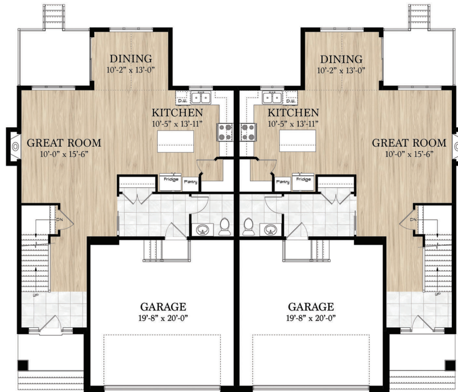
Main Floor Plan Living Area: 1753 sq. ft.
