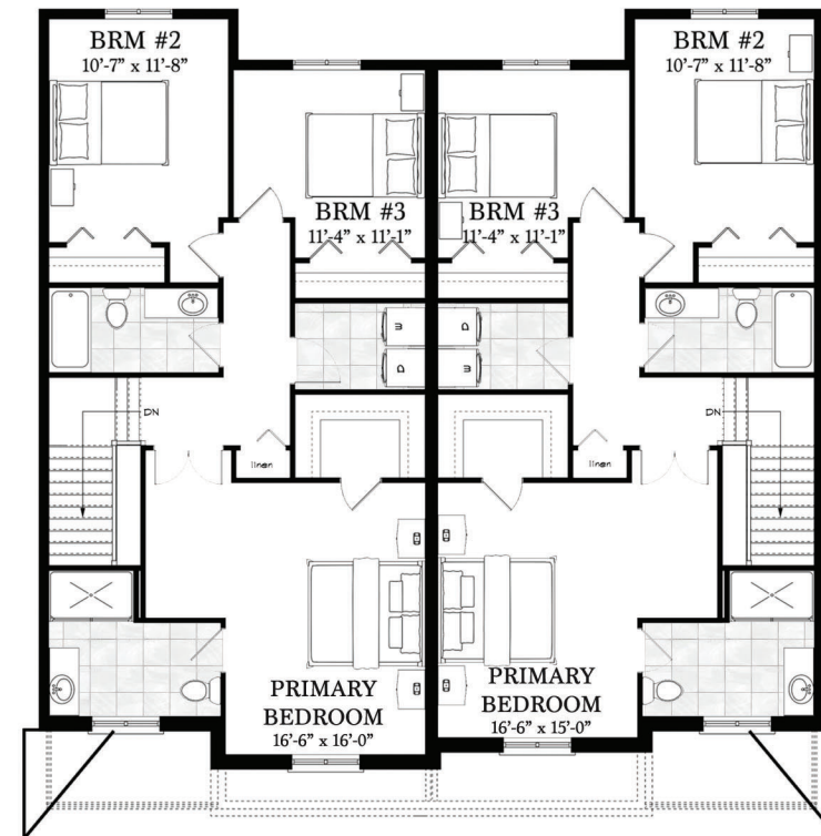
Second Floor Plan Option A Option B
